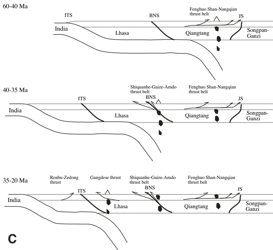
Figure 15 (continued). (C) Slab rollback of Indian plate after collision between India and Asia. ITS—Indus Tsangpo suture; JS—Jinsha suture.
