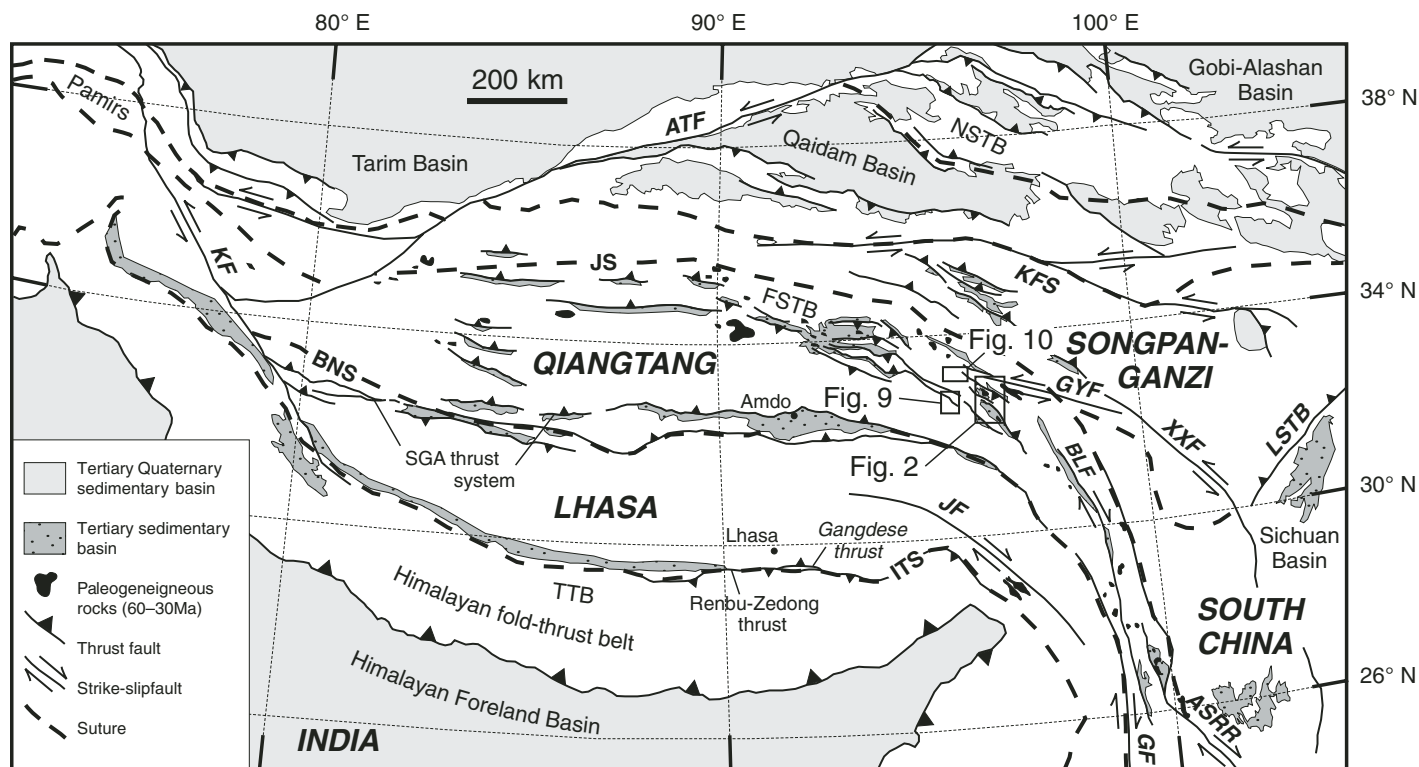
Figure 1. Simplified tectonic map of the Tibetan Plateau. Shown are sutures (JS—Jinsha suture; BNS—Banggong-Nujiang suture; ITS—Indus Tsangpo suture), major faults (KF—Karakorum fault; ATF—Altyin Tagh fault; KFS—Kunlun fault system; GYF—Ganzi-Yushu fault; XXF—Xianshuihe-Xiaojiang fault system; LSTB—Longmen Shan thrust belt; ASRR—Ailao Shan-Red River shear zone; GF—Gaoligong fault; JF—Jiali fault; BLF—Batang-Lijiang fault system), general locations of the five major Cenozoic thrust belts within the Himalaya-Tibet orogen (TTB—Tethyan thrust belt; Gangdese and Renbu-Zedong thrusts; SGA—Shiquanhe-Gaize-Amdo thrust system; FSTB—Fenghuo Shan thrust belt; NSTB—Nan Shan thrust belt), Tertiary-Quaternary sedimentary basins within and along the periphery of the Tibetan Plateau, and the distribution of Paleogene igneous rocks in northern Tibet (modified from Yin and Harrison, 2000).
