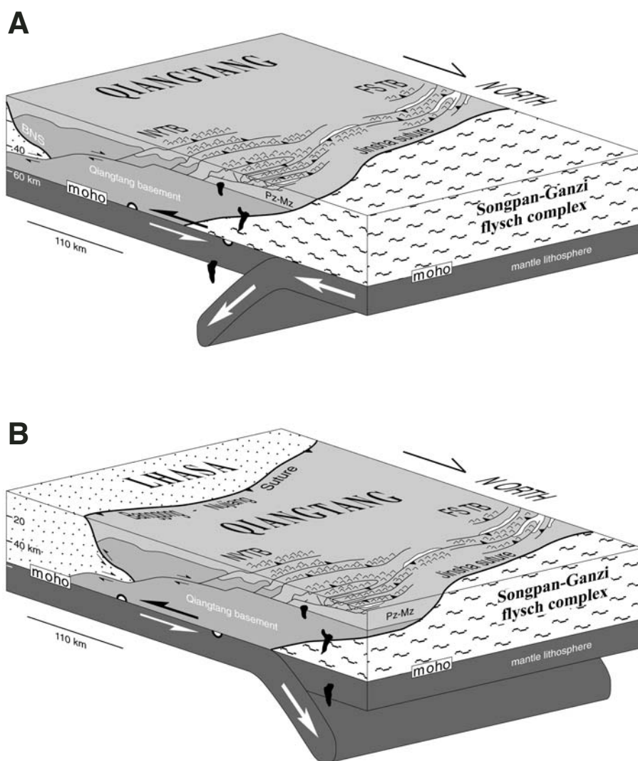
Figure 15. Alternative block models for subduction of mantle lithosphere beneath Qiangtang during Paleogene crustal shortening. (A) Subduction of the Songpan-Ganzi terrane from the north. (B) Subduction of the Lhasa terrane from the south (NYTB—Yushu-Nangqian fold-thrust belt; FSTB—Fenghuo Shan fold-thrust belt; BNS—Banggong-Nujiang suture; Pz-Mz—Paleozoic-Mesozoic strata). (Continued on following page.)
